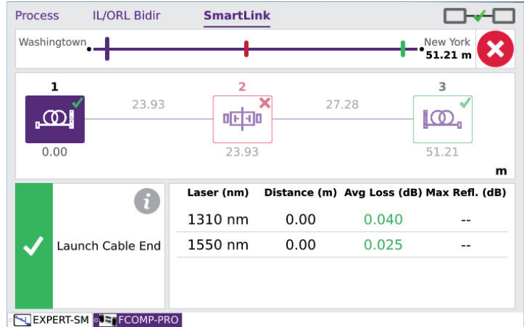
Results: Bidir OTDR events characterization
