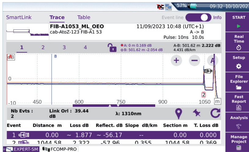
Results: unidir. Traces in Expert-OTDR app
